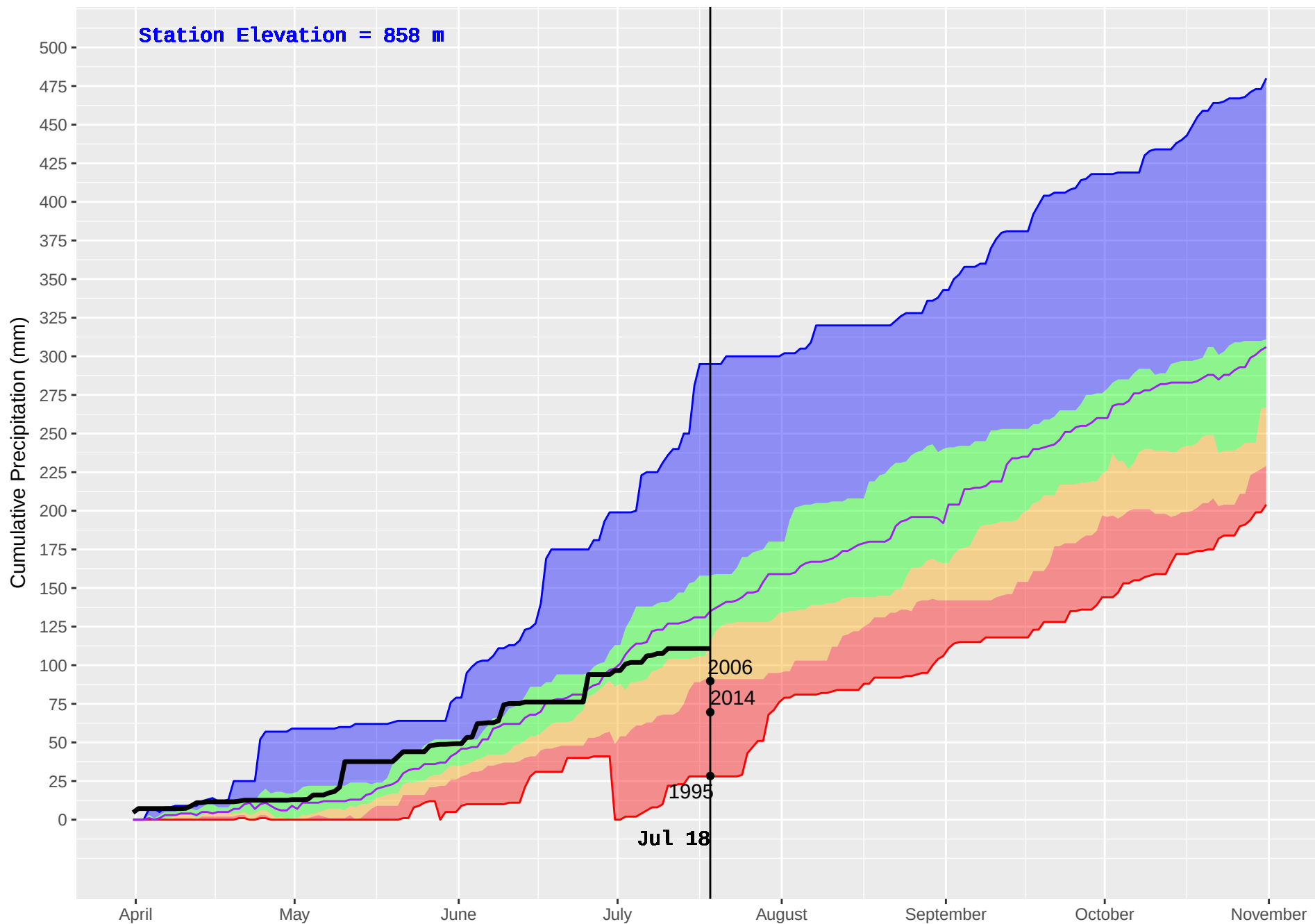
BEDNESTI (175) : Historical (1993–2016) and Current (2018) Daily Cumulative Precipitation
