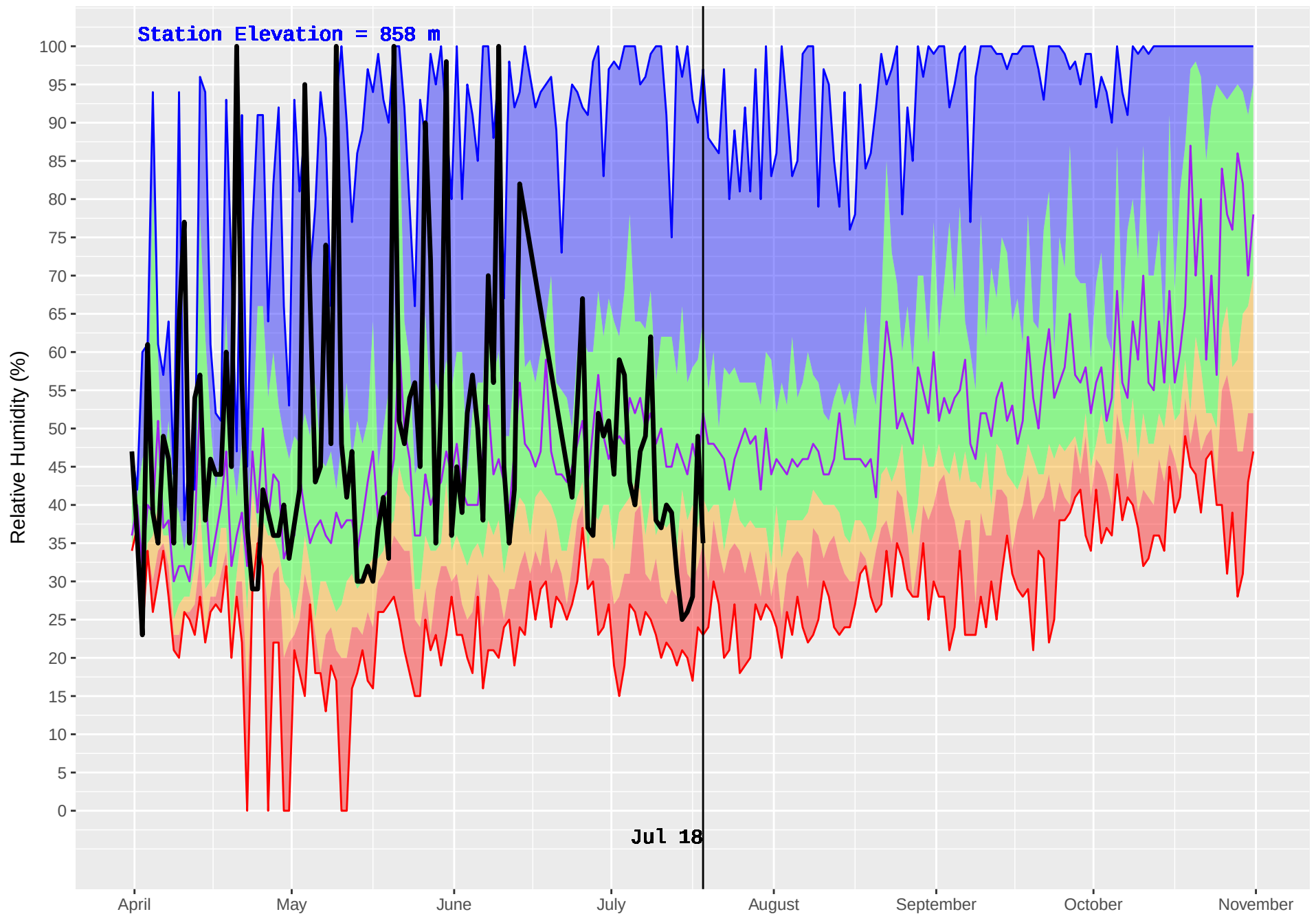
BEDNESTI (175) : Historical (1993–2016) and Current (2018) Daily Relative Humidity
