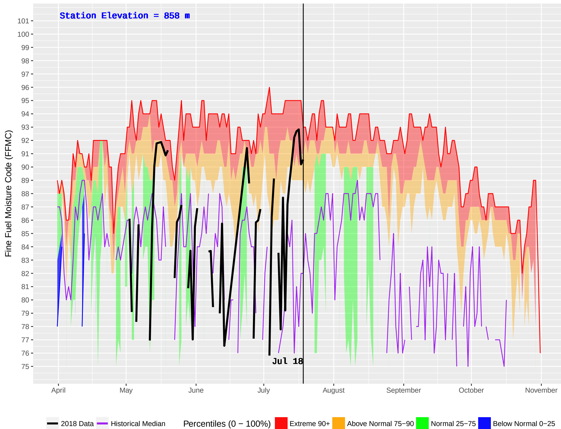
BEDNESTI (175) : Historical (1993–2016) and Current (2018) Daily Fine Fuel Moisture Code (FFMC)
