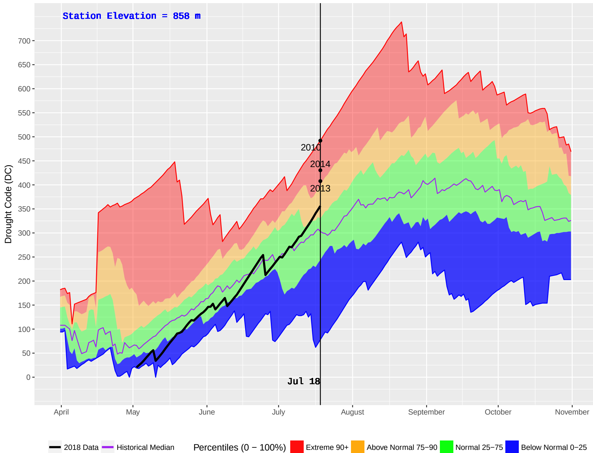
BEDNESTI (175) : Historical (1993–2016) and Current (2018) Daily Drought Code (DC)
