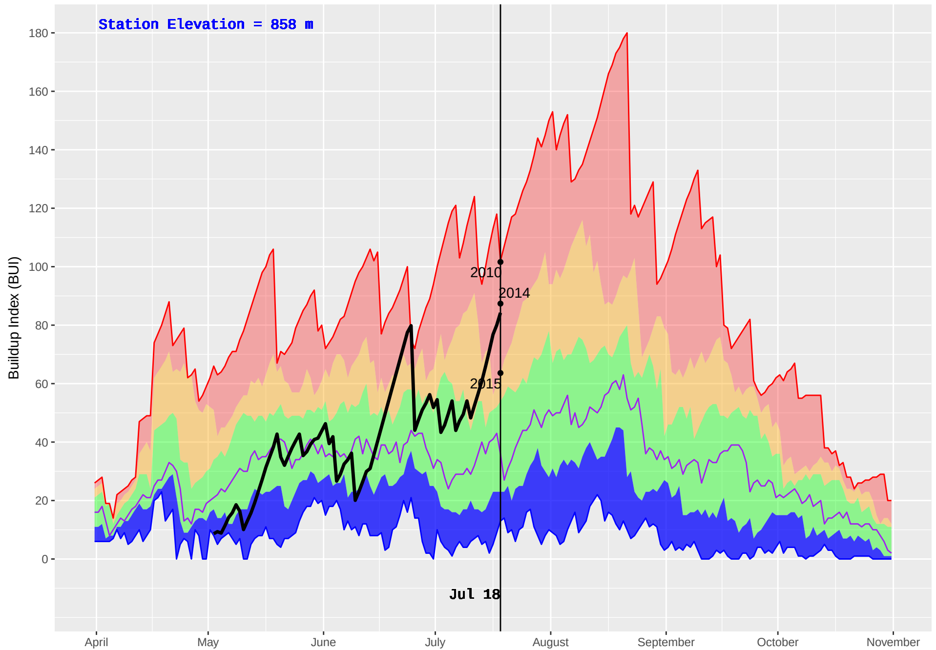
BEDNESTI (175) : Historical (1993–2016) and Current (2018) Daily Buildup Index (BUI)
