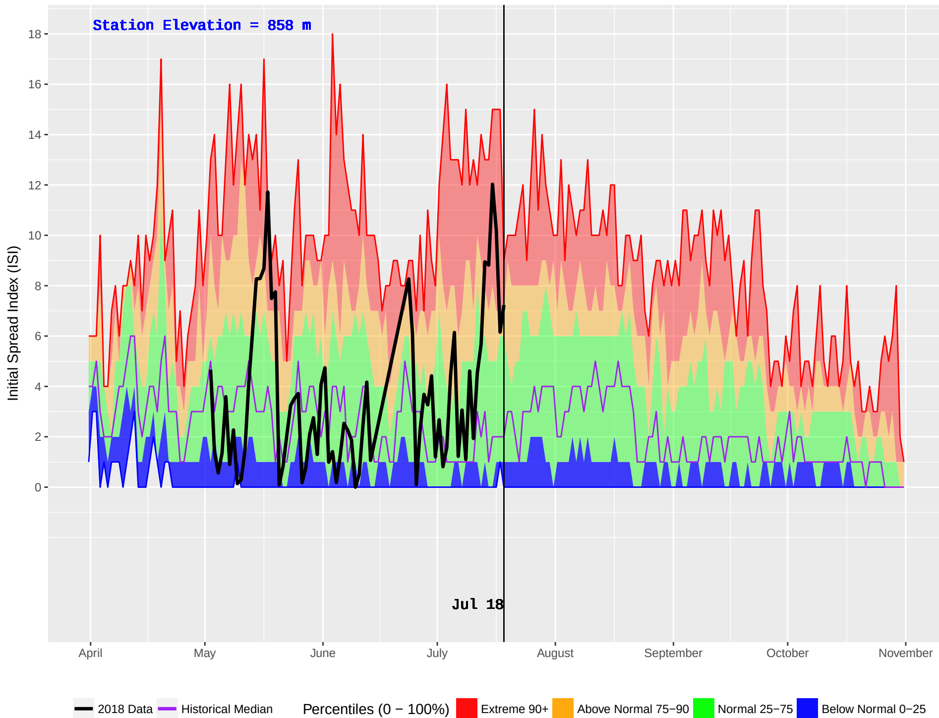
BEDNESTI (175) : Historical (1993–2016) and Current (2018) Daily Initial Spread Index (ISI)
