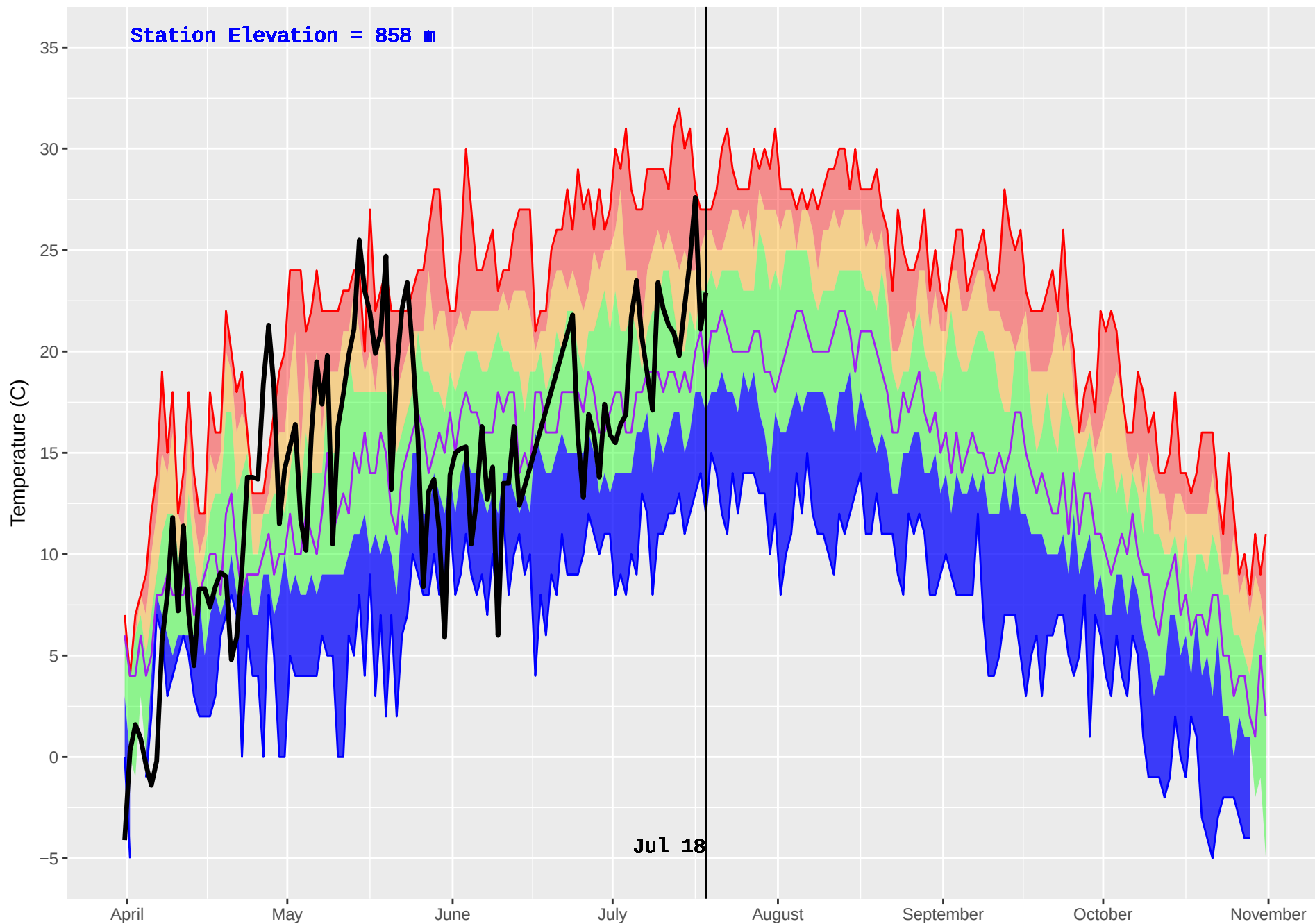
BEDNESTI (175) : Historical (1993–2016) and Current (2018) Daily Temperature
