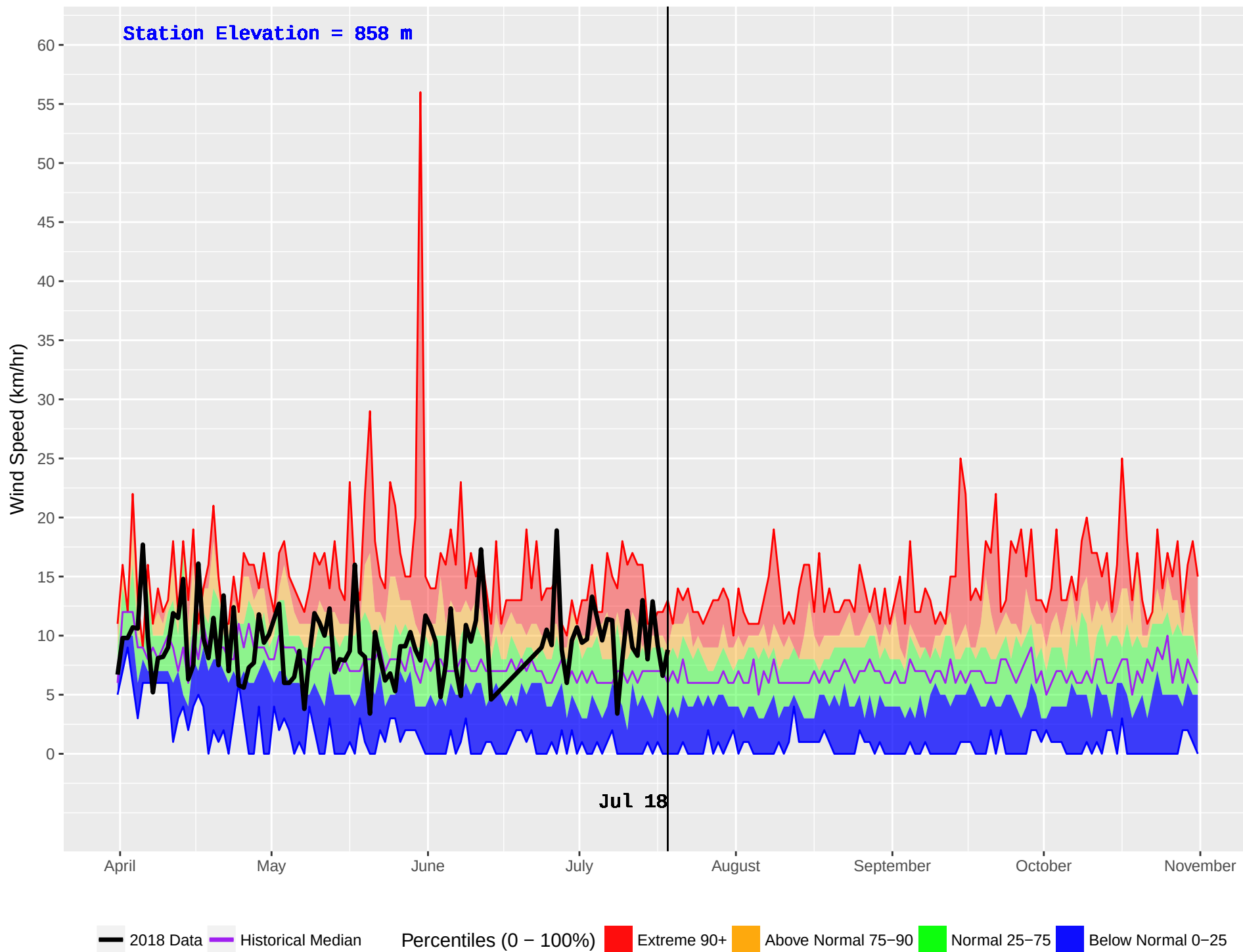
BEDNESTI (175) : Historical (1993–2016) and Current (2018) Daily Wind Speed
