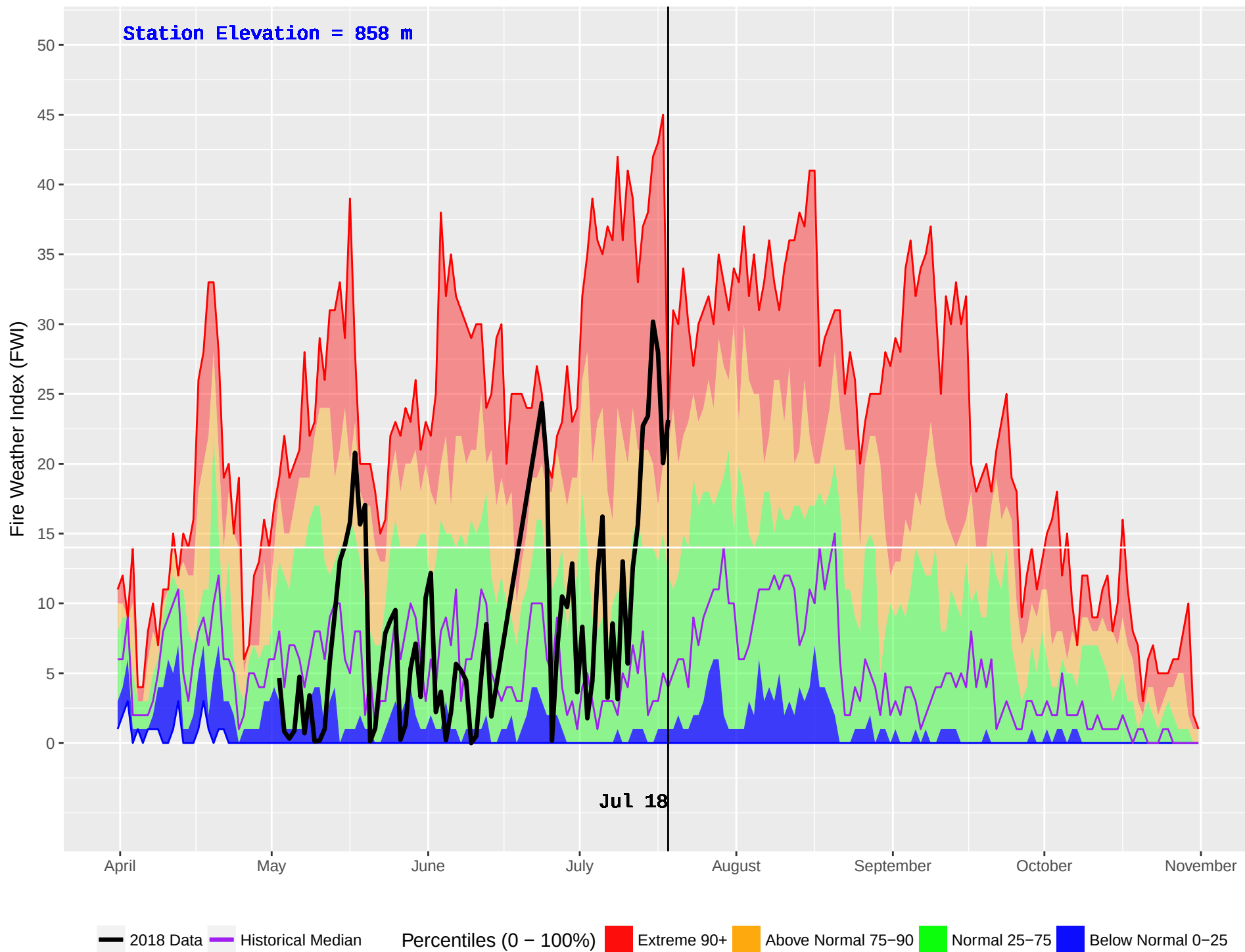
BEDNESTI (175) : Historical (1993–2016) and Current (2018) Daily Fire Weather Index (FWI)
